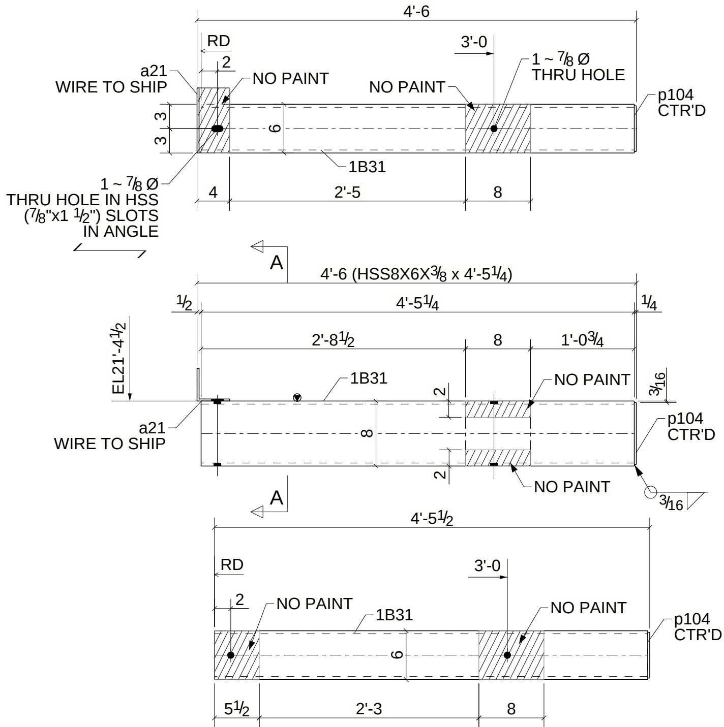
ONE - HSS GIRT - 1B31
